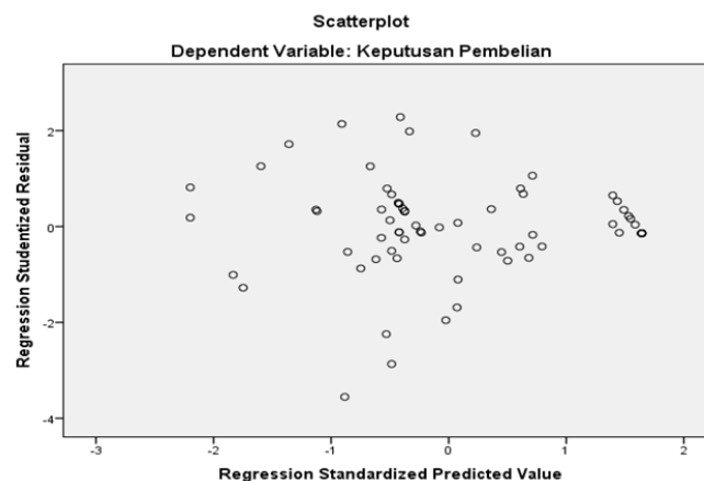
Gambar 6. Heteroscedacity Test
