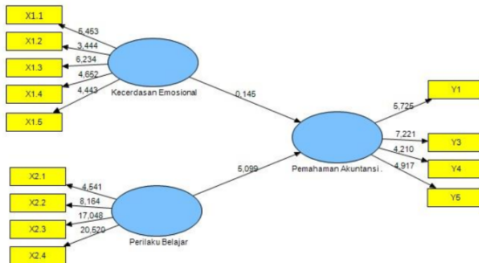
Figure 1: Hypothesis Test Curve
